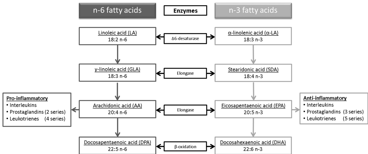
Fig. 2. A simplified overview of the polyunsaturated fatty acid pathway. Omega-6 and omega-3 fatty acids are taken up as essential fatty acids (EFAs; LA and α-LA) through food consumption. Due to enzyme competition, the fatty acids will be converted into the long-chain PUFAs AA and DHA, depending on the amount of EFAs that are available. Due to the competition there will be an adverse effect: an increase in omega-6 will lead to a decrease in omega-3 and vice versa.
