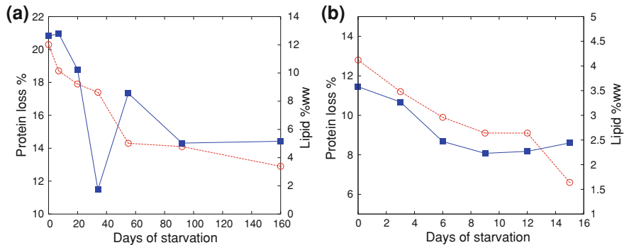
Fig. 6.2 Values of protein (% BM, circles) and lipid (% BM, squares) during a 160 days of starvation in red sea bream (Woo and Fung 1981) and b 15 days (Gunasekera et al. 2001)
