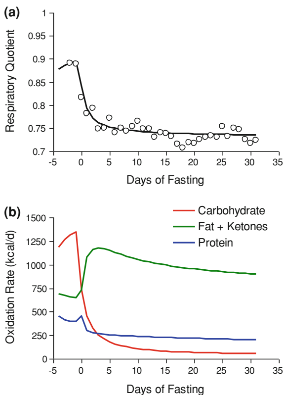
Fig. 22.4 a Measured respiratory quotient ( \circ ) in Benedict's subject during starvation along with the computational model prediction ( curve ). b Computational model predictions of the rates of carbohydrate, fat, ketone, and protein oxidation during starvation
