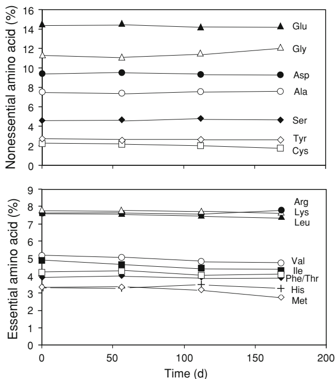
Fig. 8.5 Amino acid composition in the bodies of five snake species and a lizard subjected to complete fasting for 168 days at 27°C and 12L:12D. The species are the same as in Fig. 8.1
