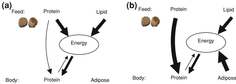
Fig. 6.6 Utilization of dietary components for a lean fish, where most of the energy to protein synthesis is satisfied from dietary fat and protein and b fish with high fat levels, which can supply the fuel to protein synthesis from its adipose cells. The width of the arrows indicates the flux size
